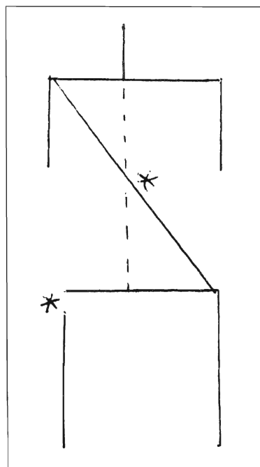
Asymmetrical Vectors
