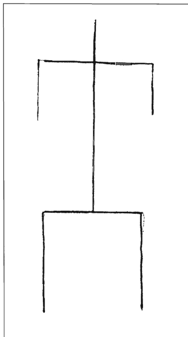
Normal Vectors
